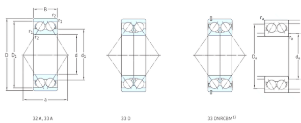
Bearing No. 3205ATN9
