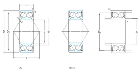
Bearing No. 3205A-2RS1
