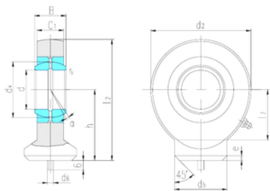
Bearing No. SK12E
