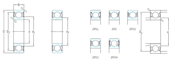
Bearing No. W628/6-2Z
