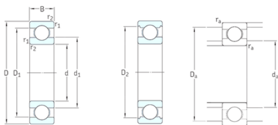
Bearing No. W627/6X
