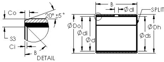
Bearing No. AST40 0606
