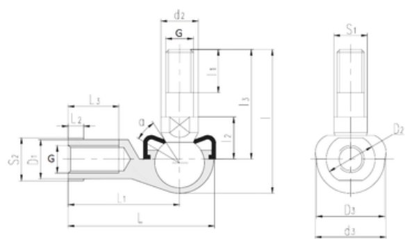
Bearing No. SQ8-RS
