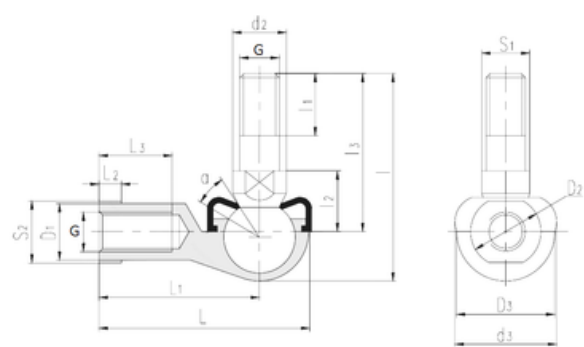
Bearing No. SQ16-RS
