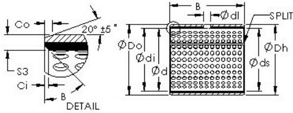
Bearing No. AST20 8540
