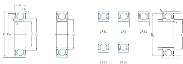
Bearing No. W638/2.5-2Z
