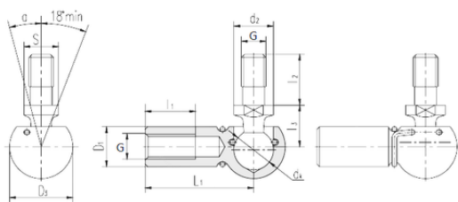
Bearing No. SQG12
