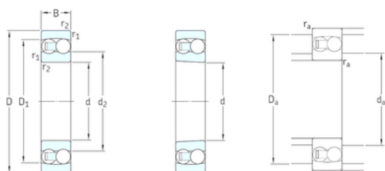
Cylindrical bore
