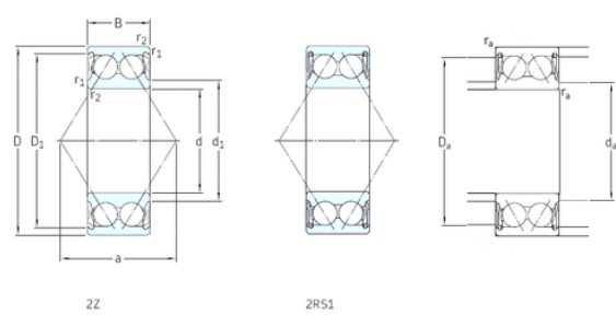
Bearing No. 3200A-2RS1
