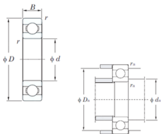
Bearing No. 6803
