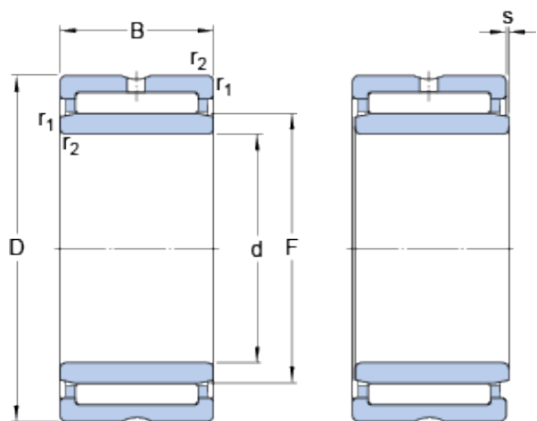
Bearing No. NKI 35/30
