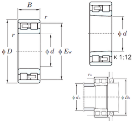
Bearing No. NN3006K
