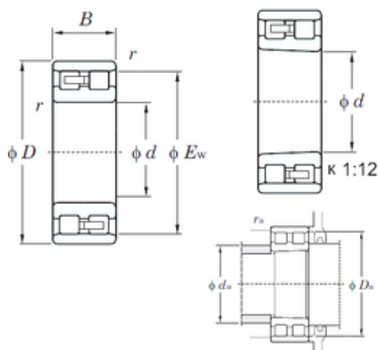
Bearing No. NN3060K
