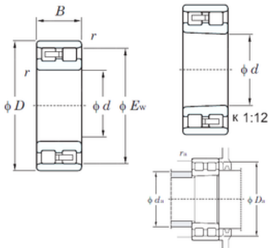
Bearing No. NN3072K
