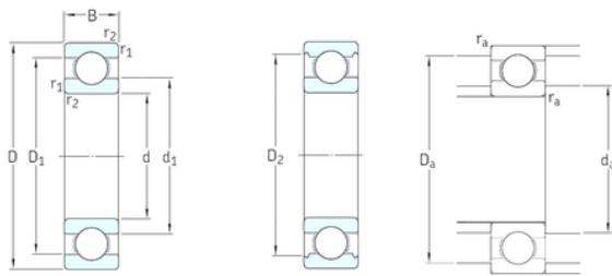
Bearing No. 628
