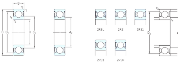
Bearing No. 627-RSH
