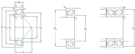
Bearing No. 7232BCBM
