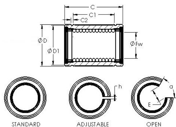
Bearing No. LBB 16 AJ
