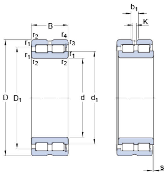
Bearing No. NNCF 5034 CV
