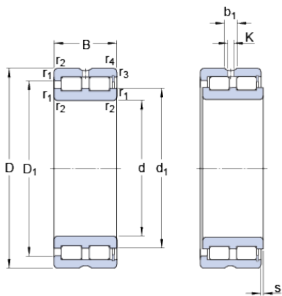
Bearing No. NNCF 4914 CV
