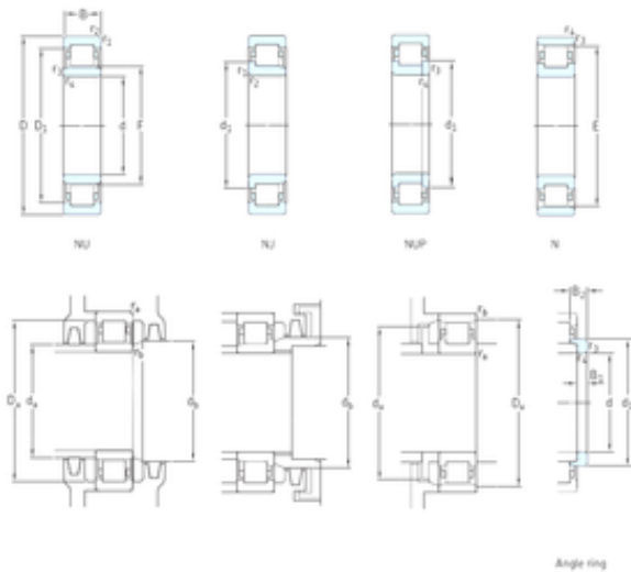
Bearing No. NJ2306ECP
