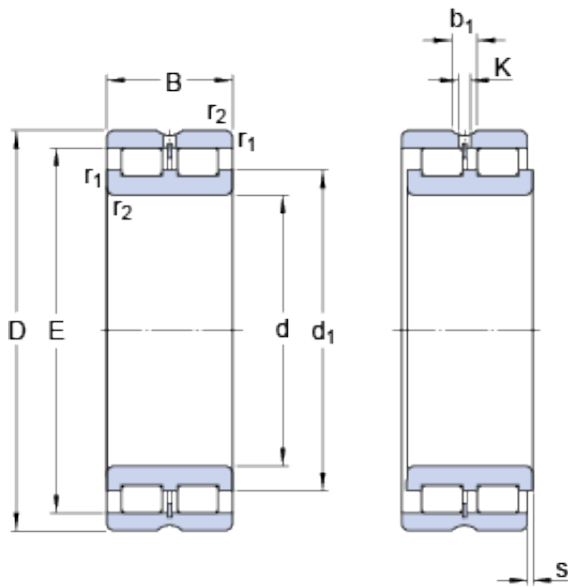
Bearing No. NNCL 4940 CV
