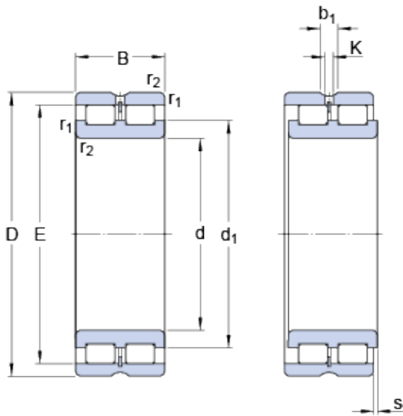
Bearing No. NNCL 4934 CV
