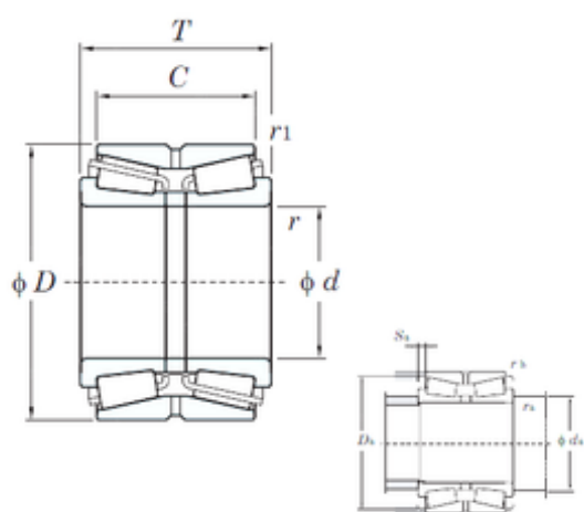
Bearing No. 46T32226JR/117,5
