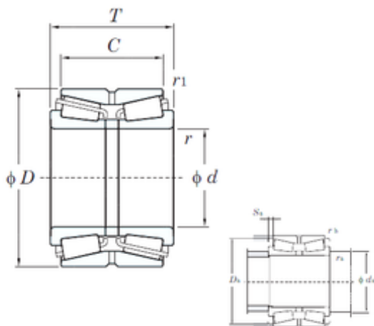
Bearing No. 46T32220JR/87
