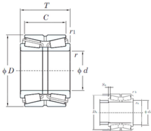
Bearing No. 46T30319JR/85
