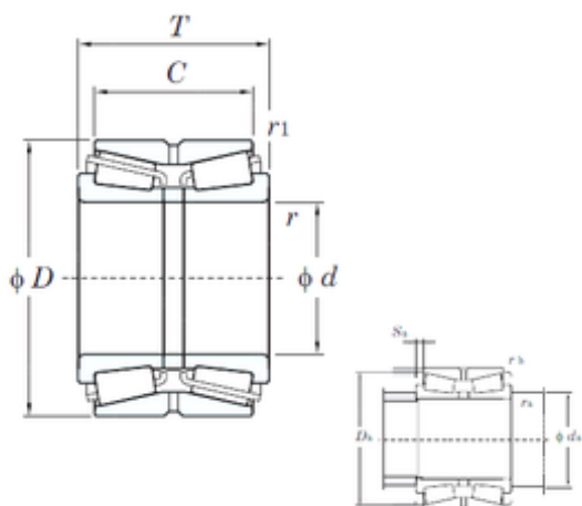
Bearing No. 46320A
