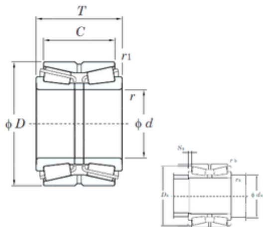
Bearing No. 46288A
