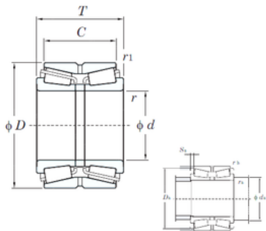
Bearing No. 46284A
