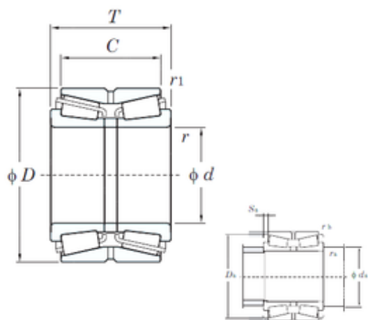
Bearing No. 46268
