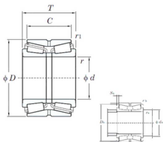
Bearing No. 462/500
