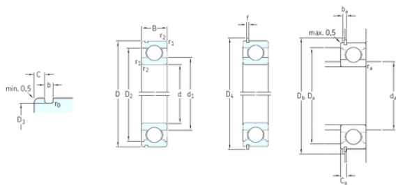
Bearing No. 6214NR
