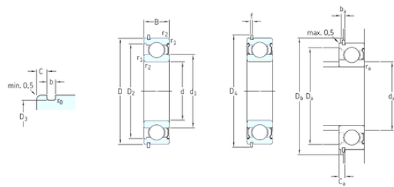
Bearing No. 6214-2ZNR
