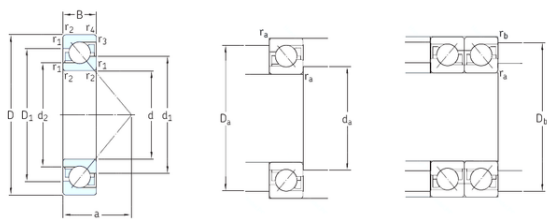
Bearing No. 7314BEP
