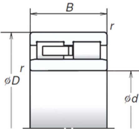
*NNU49 Cylindrical Bore
