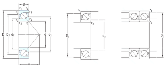
Bearing No. 7315BECBM
