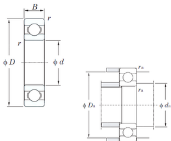
Bearing No. 6210R
