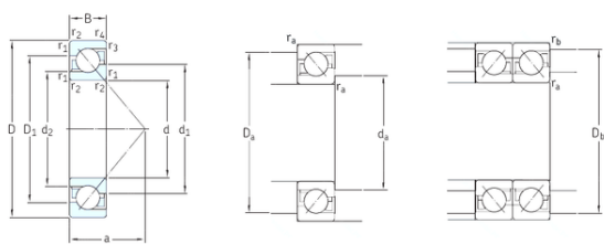
Bearing No. 7322BECBP
