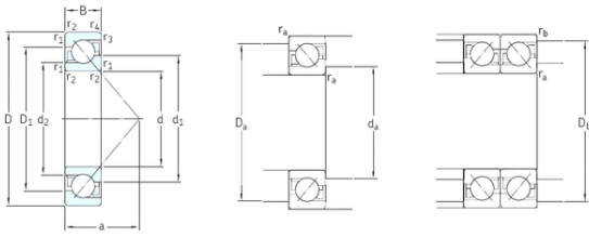
Bearing No. 7322BECBM
