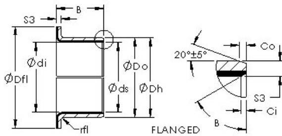
Bearing No. AST11 F18170
