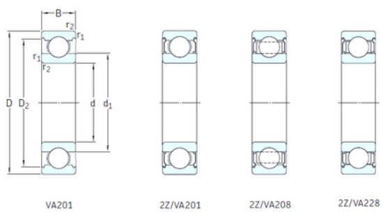
Bearing No. 6205/VA201
