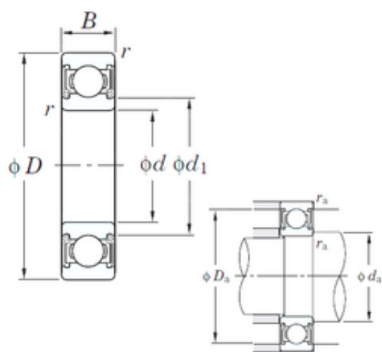
Bearing No. 6204 2RD C3
