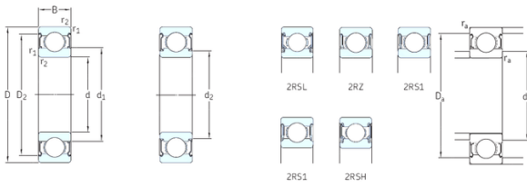
Bearing No. 6202-2Z
