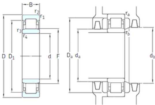
Bearing No. NU1015M/HC5C3
