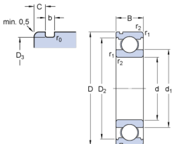
Bearing No. 6202 N
