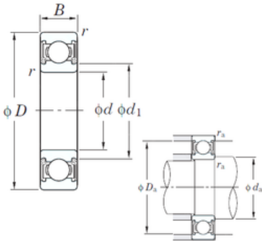
Bearing No. 6202 2RD C3
